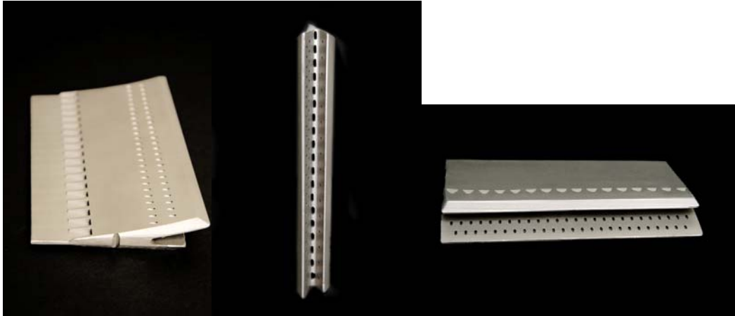
Figures 4 and 5. The 7FA Trailing Edge Replacement Coupon with cooling hole geometry made with the EDM process.
